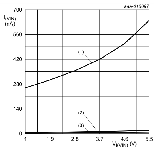
Fig 9. Typical supply current versus input voltage on pin VIN
