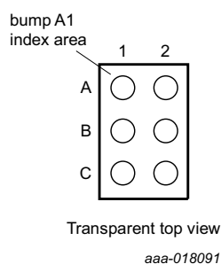
Fig 3. Pin configuration for WLCSP6
