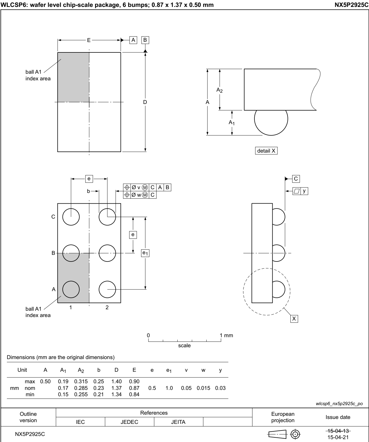
Fig 23. Package outline NX5P2925C
